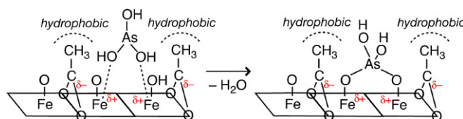
Fig. 9. Proposed promoted sorption mechanism of low concentrations of arsenite on acetate-exchanged FeO x (OH) y heated at 423 K.
